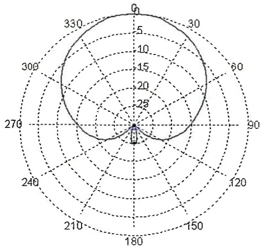
Azimuth (H-field) radiation pattern
