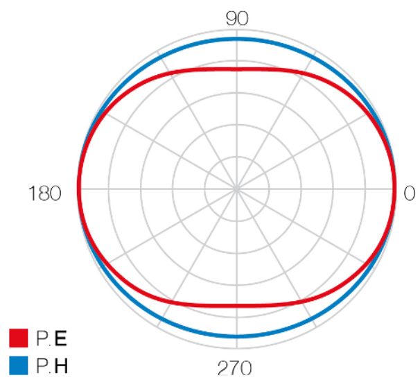
Radiation pattern
